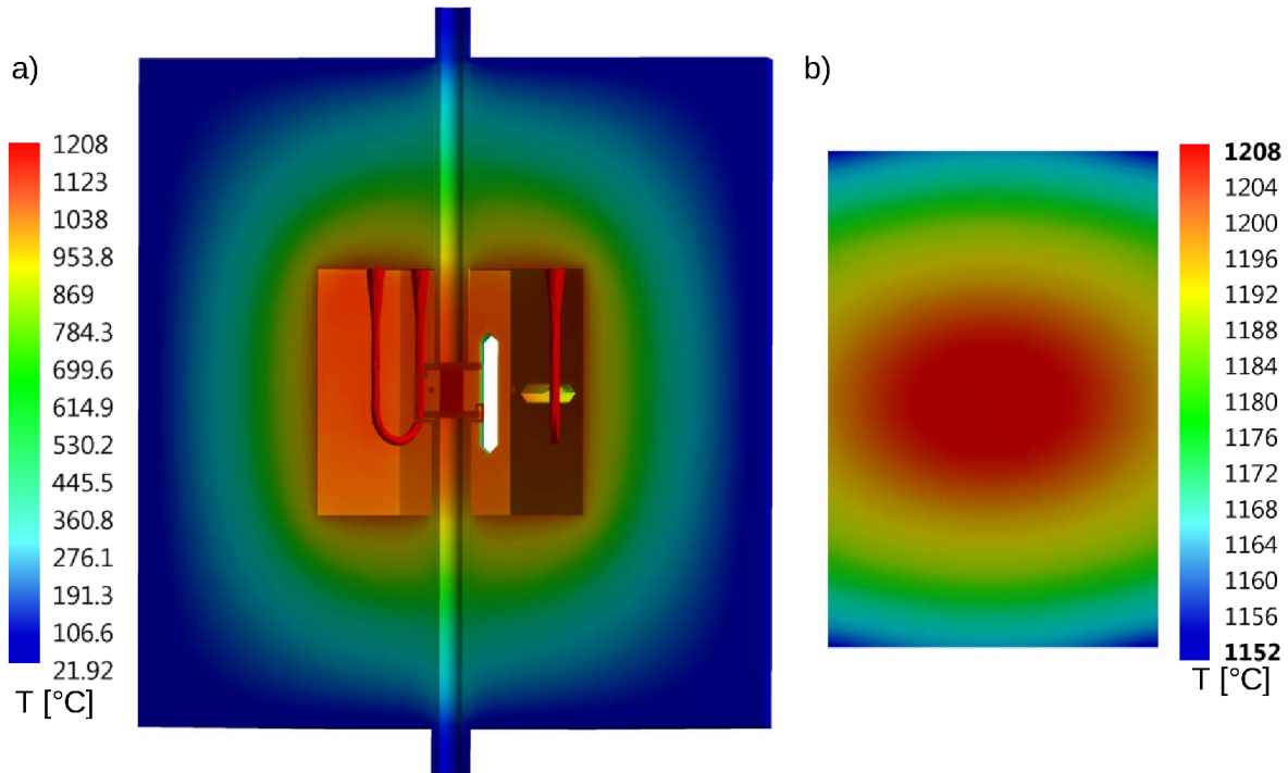
3 Figure 7: Simulation result of temperature distribution in loading dilatometry under 4 E_{rms} = 28 \text{ V/cm} with T_{furnace} = 1188 \text{ }^{\circ}\text{C} : a) isometric view; b) detailed view of the sample.
