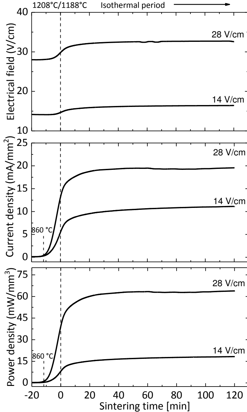
1 2 Figure 10: Electrical field, power density and current density over sintering time under 3 E_{rms} = 14 V/cm and 28 V/cm.
